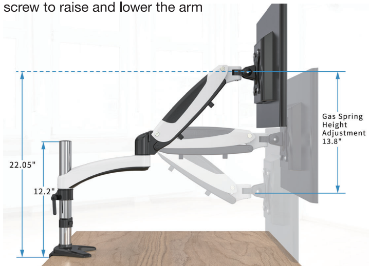
The wrench adjusts the inner damping screw to raise and lower the arm
